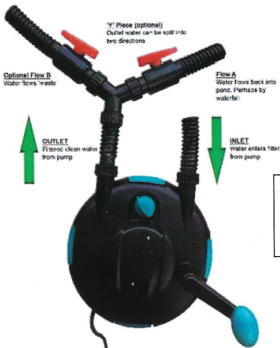
Image showing overview of Filter when a small Y Distributor is attached
